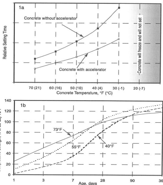
Figure 1 Effect of Temperature on Set Time (1a)
